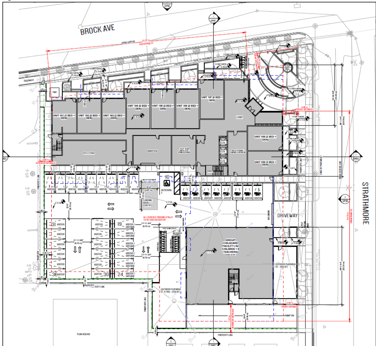
Figure 6: Site Plan
